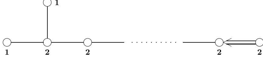
Figure 5: Dynkin diagram A_{2n-1}^{(2)} ( n \geq 3 )
